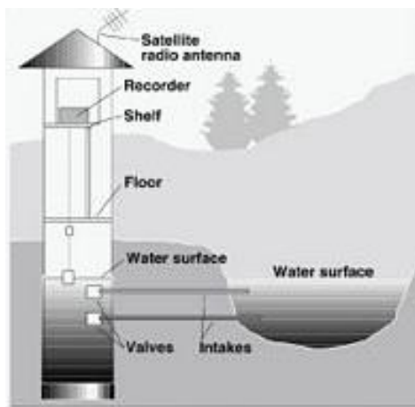
Figure 5: Typical Modern USGS Stream Gage
