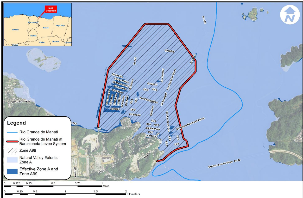
Figure 3: Natural Valley Procedure
