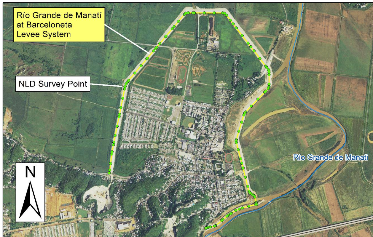
Figure 1: Río Grande de Manatí at Barceloneta Levee System Location
