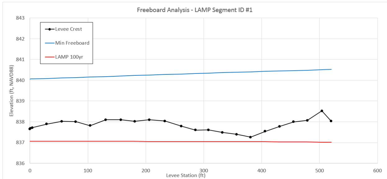
Figure 7: First Pass results for Susquehanna River - Levee Segment ID #0 and #1
