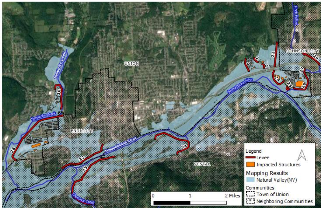
Figure 5: First Pass results for Town of Union Levees with Structures Impacted from Natural Valley Mapping
