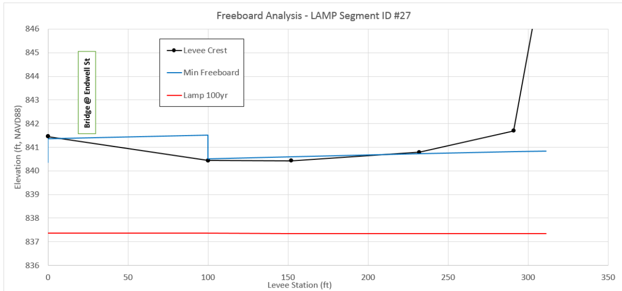
Figure 10: First Pass results for Susquehanna River - Levee Segment ID #26 and #27
