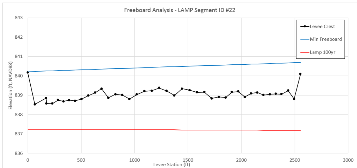
Figure 8: First Pass results for Susquehanna River - Levee Segment ID #2 and #22
