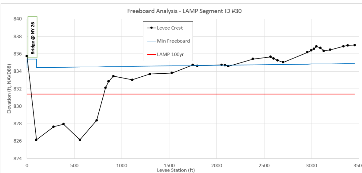
Figure 6: First Pass results for Nanticoke Creek - Levee Segment ID #28 and #30
