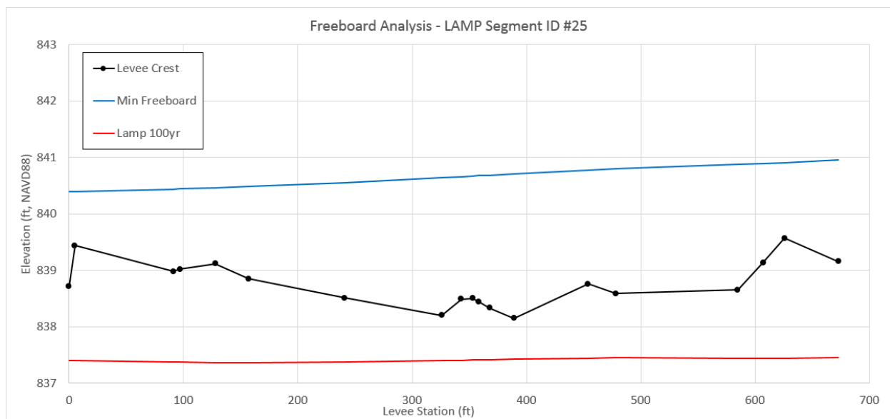
Figure 9: First Pass results for Susquehanna River - Levee Segment ID #24 and #25
