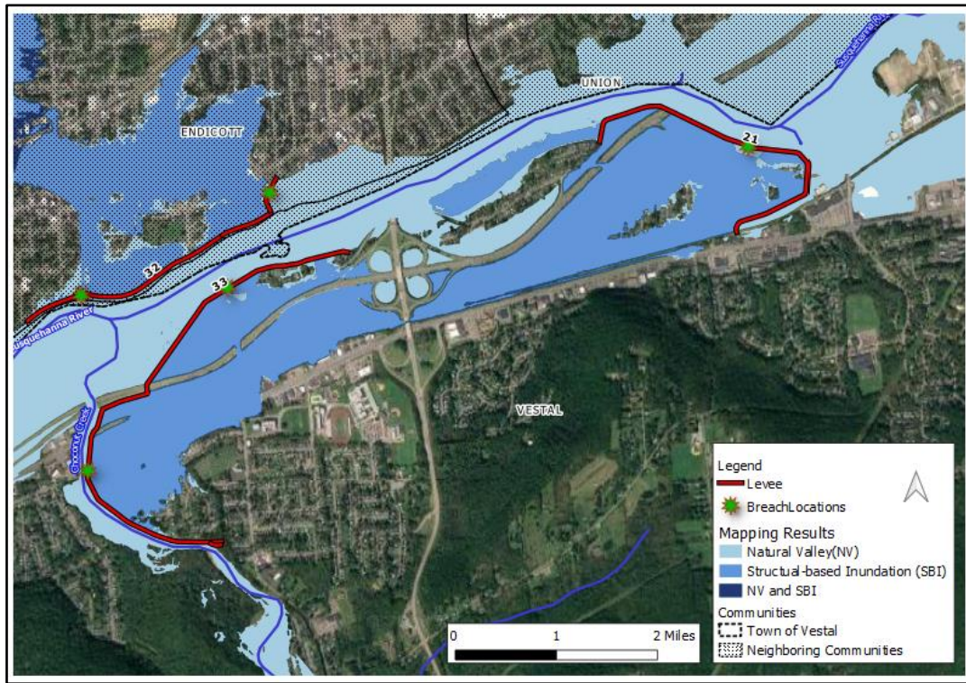
Figure 4: Structural-based Inundation Procedure Mapping
