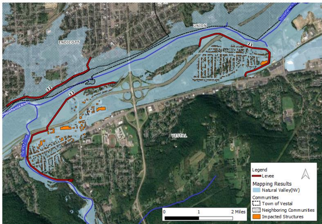
Figure 5: First Pass results for Susquehanna River/Choconut Creek Impacted from Natural Valley Mapping
